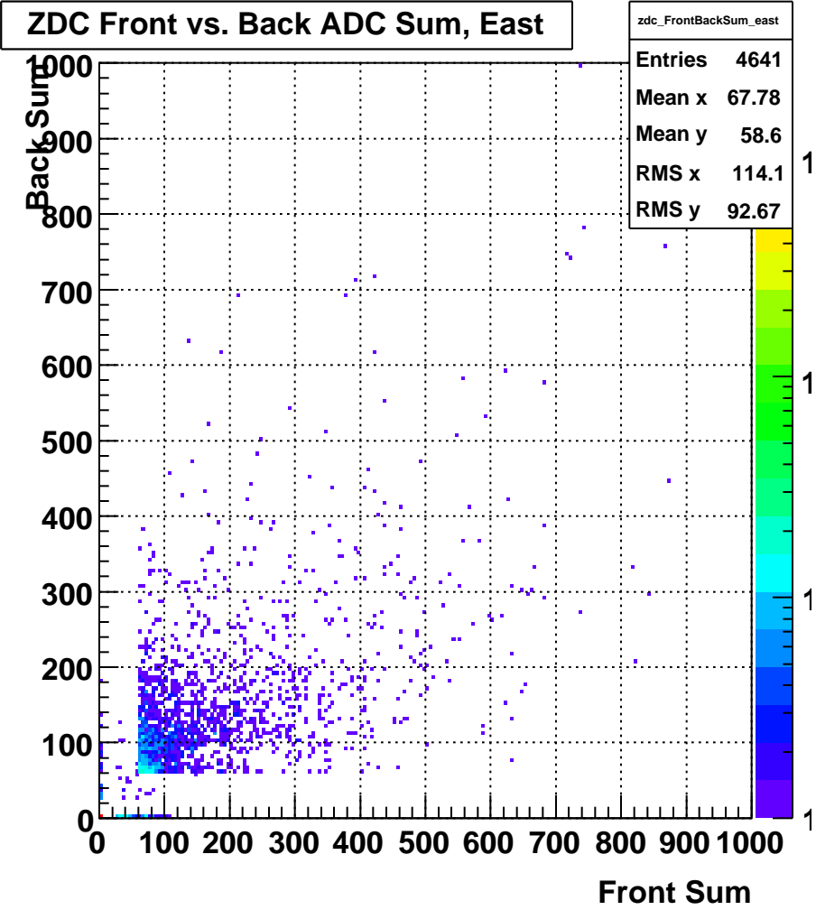
ZDC Front vs. Back Sum (run 10109013)
