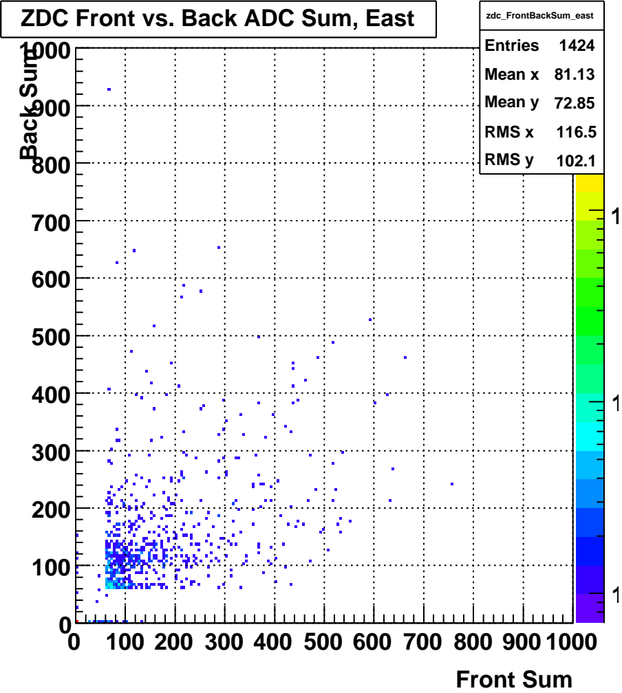
ZDC Front vs. Back Sum (run 10108015)
