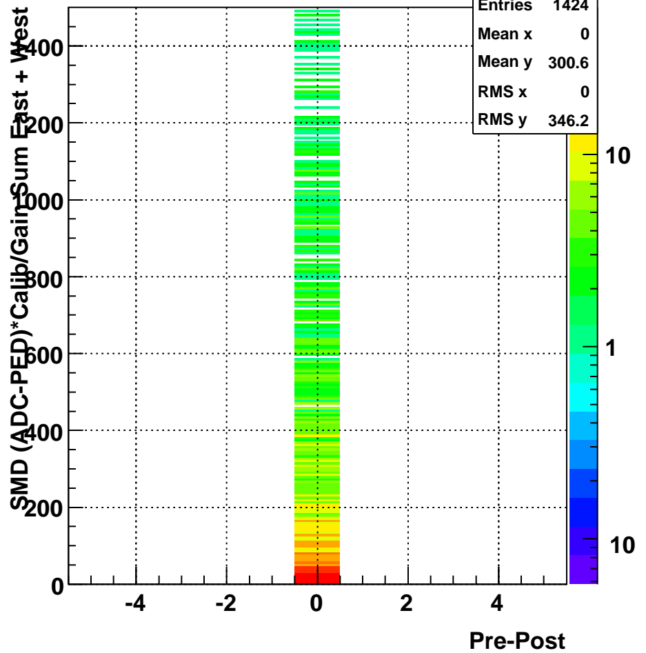
ZDC SMD ADC Corr Sum vs. Pre-Post
