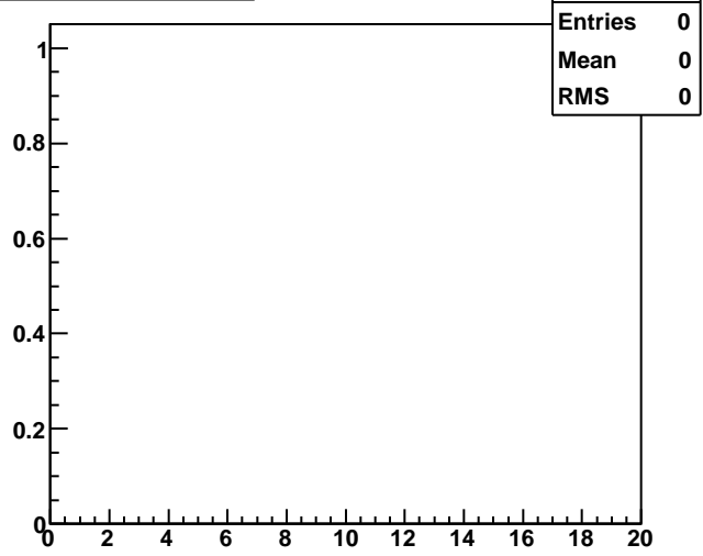
pair_towerEnergy2
