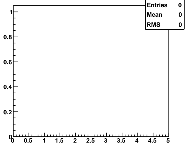
pair_p2/pair_towerEnergy2
