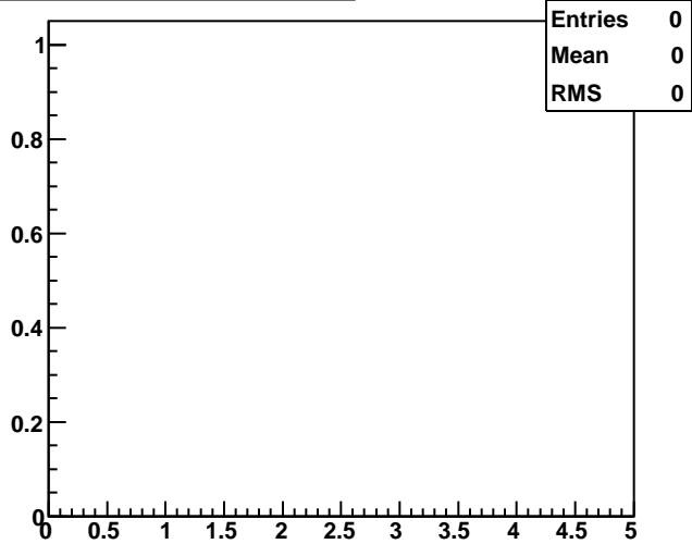
pair_p1/pair_towerEnergy1
